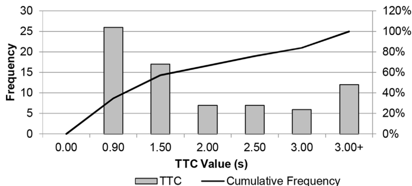
Fig. 6. TTC frequency and cumulative frequency distributions for all incidents.
