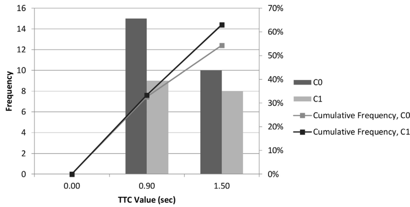
Fig. 7. TTC frequency and cumulative frequency distributions, by curb radius treatment level.
