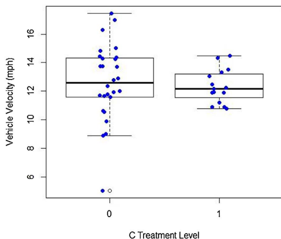
Fig. 10. Boxplot and scatterplot of vehicle velocities for curb radius treatment levels.
