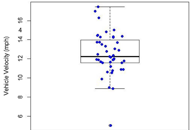
Fig. 9. Boxplot and scatterplot of vehicle velocities for all moderate- & high-risk incidents.
