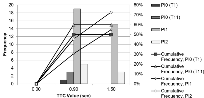
Fig. 8. TTC frequency and cumulative frequency distributions by protected intersection treatment level.
